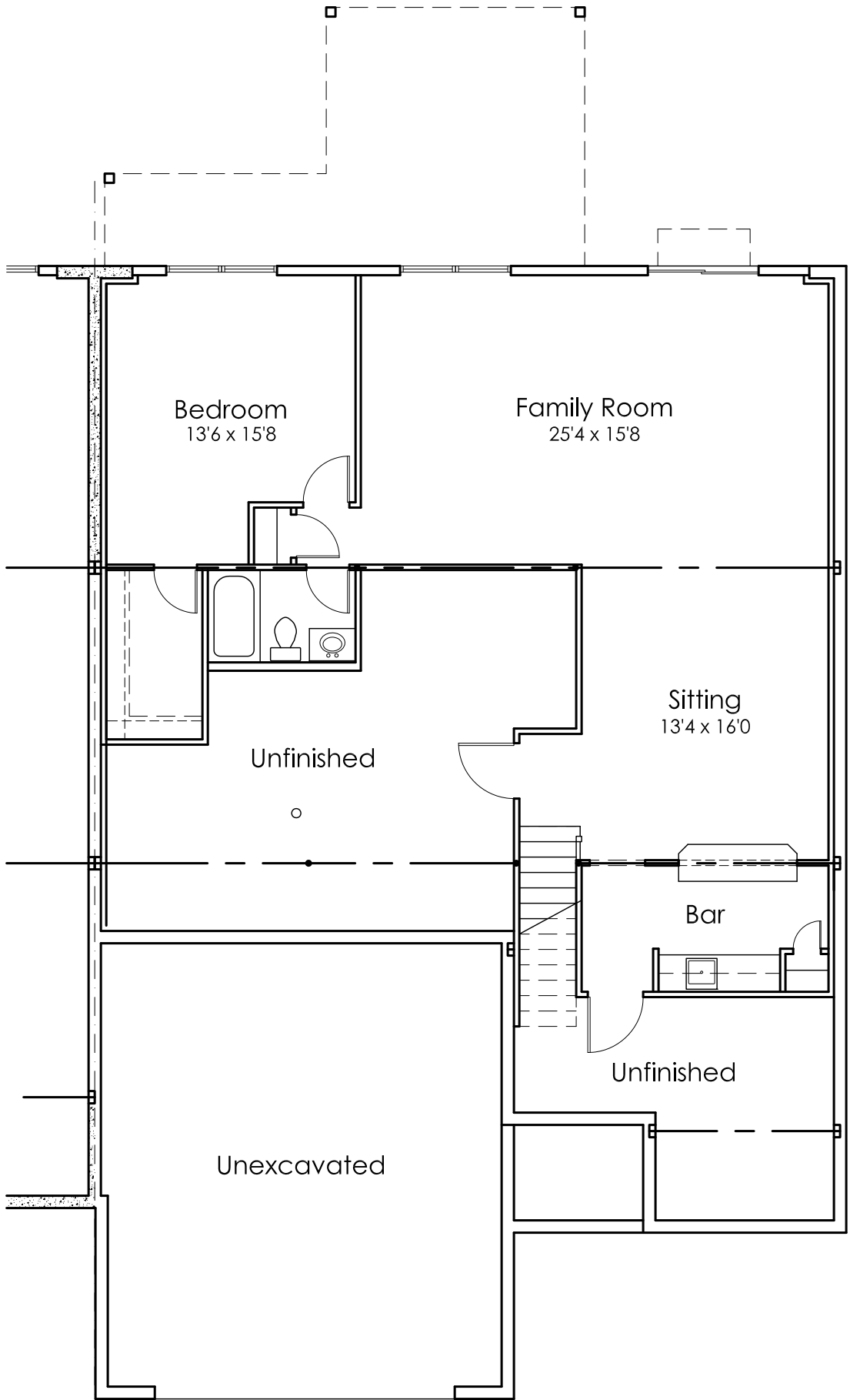
1 Basement Plan
