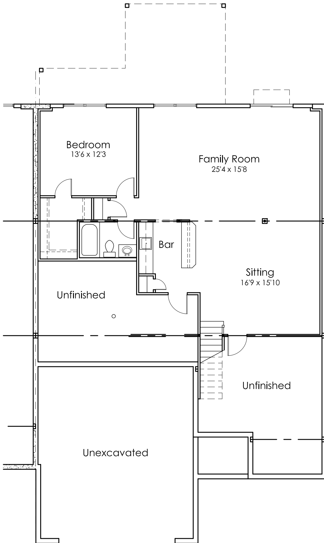
3 Basement Plan
